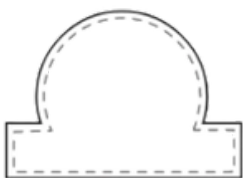
custom
