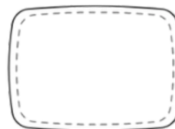
rounded rectangle
