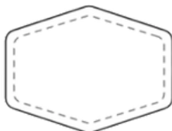
hexagon
